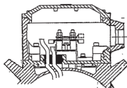
Terminal box for motors sizes 160 - 180
