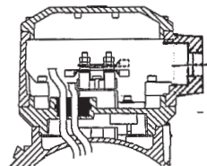
Terminal box for motors sizes 200 - 280
