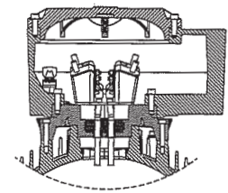
Terminal box for motors sizes 315 - 355
