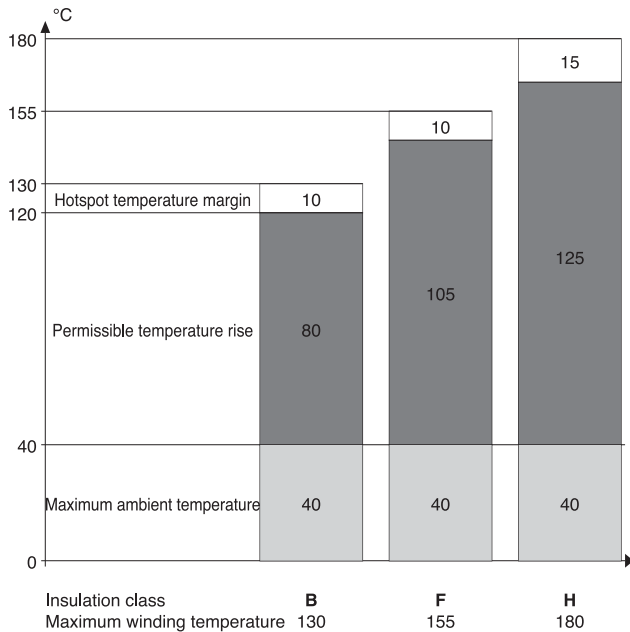
Safe margins per insulation class
